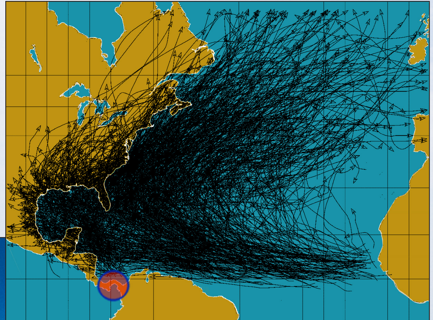
Hurricane paths from 1851 through 2004 documented by NOAA
